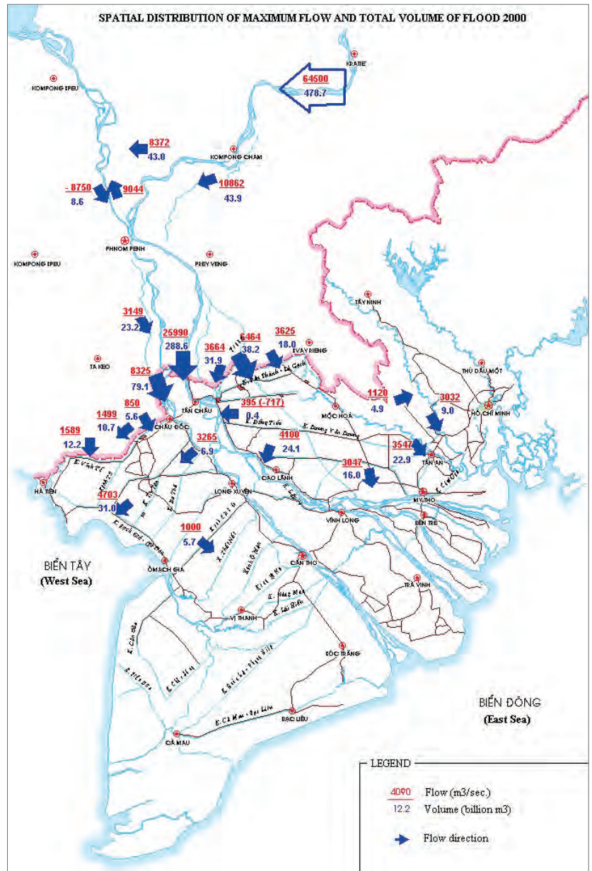
Fig. 3 Spatial distribution of the maximum flood flow and total volume of the 2000 flood from a VRSAP model simulation (source: Southern Institute for Water Resources Planning)
