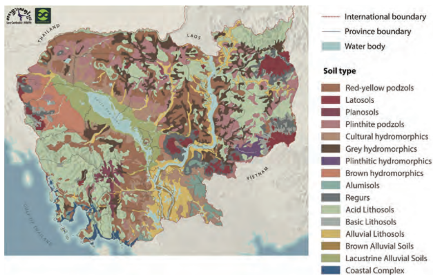
Fig. 5 Soil type map of Cambodia
