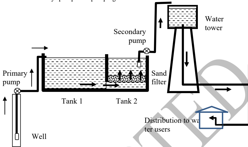
Fig. 2: Structural operation scheme of the existing water supply station
