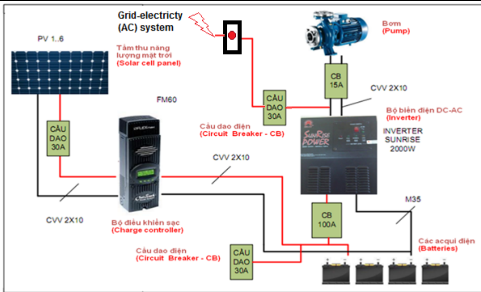
Fig. 4: Conceptual scheme of My Phung Water Supply Plant's solar power system
