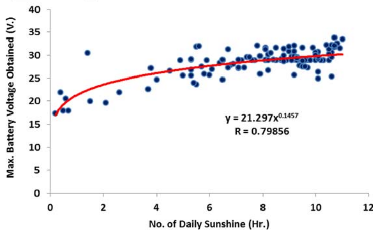
Fig. 7: Power correlation trend curve between in site max. Voltage and sunshine duration
