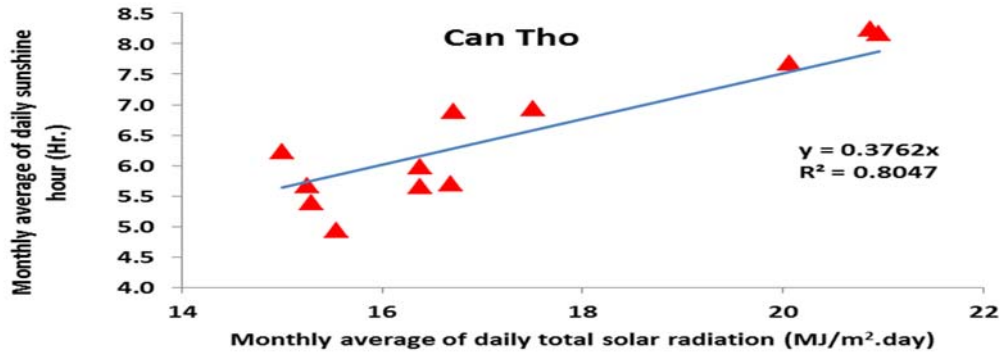
Fig. 5: Linear correlation between daily sunshine hour and daily solar radiation in Can Tho
