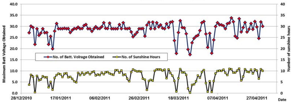
Fig. 6: Maximum Battery Voltage obtained vs. No. of sunshine hours measured in site
