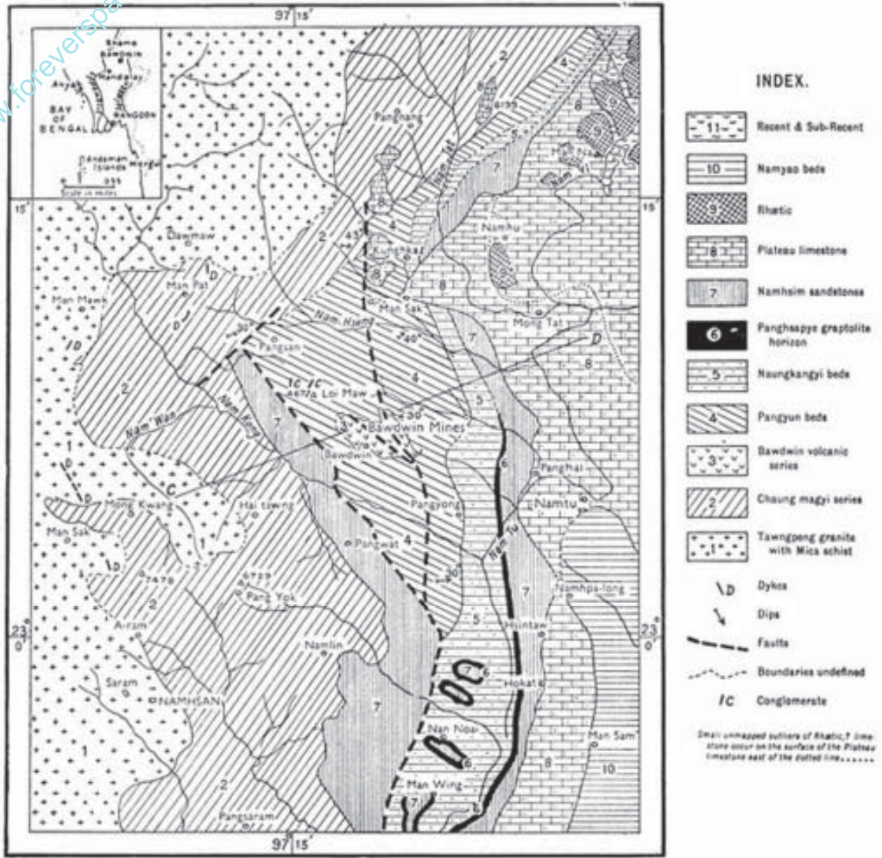
SECTION ALONG THE LINE C-D GEOLOGICAL MAP SHOWING BAWDWIN AND SURROUNDING COUNTRY. Scale, 1 inch = 4 miles.
