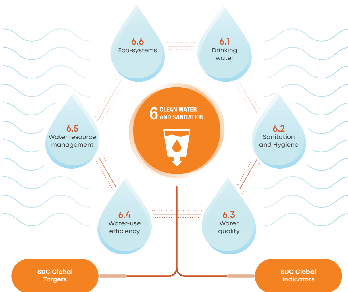
FIGURE 19: SDG 6 TARGETS AND INDICATORS FOR DRINKING WATER, SANITATION AND HYGIENE
