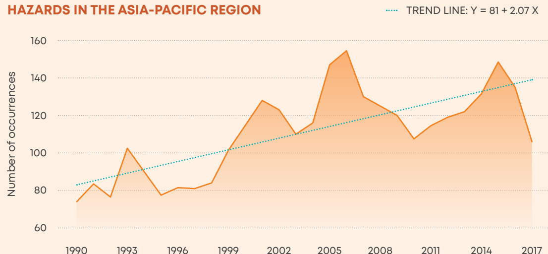
FIGURE 15: TRENDS IN THE OCCURRENCE OF CLIMATIC HAZARDS IN THE ASIA-PACIFIC REGION
