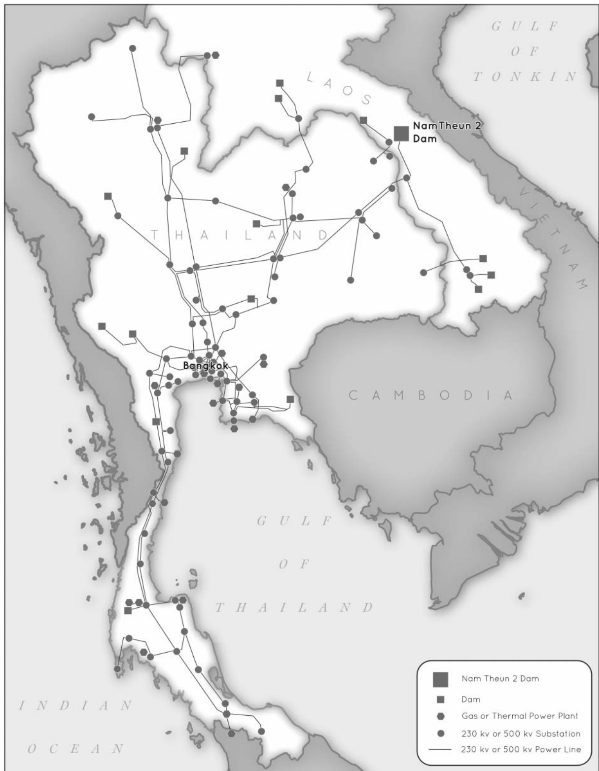
Figure 3. Map showing the electricity grid in Thailand and how it is linked to the Nam Theun 2 Hydropower Project (NT2) in central Laos.
