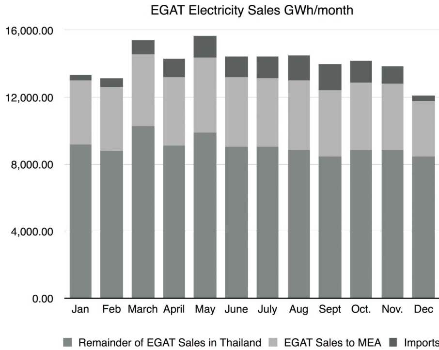
Figure 6. Electricity Generating Authority of Thailand (EGAT) energy use and imports, indicating that energy imports from Laos follow load requirements. Source: Compiled by authors based on Ministry of Energy (2014).
