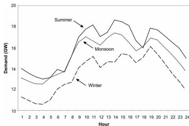
Figure 4. Daily demand profiles in Thailand, showing load patterns shifting both daily and seasonally. EGAT (2004), reprinted in Parkboom and Harrison (2008, 1442).
