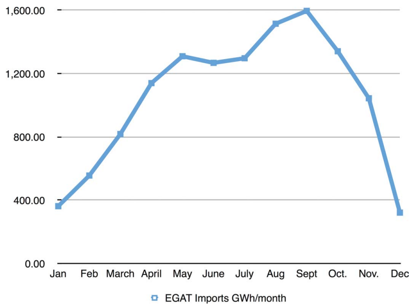
Figure 7. Electricity Generating Authority of Thailand (EGAT) energy imports per month, indicating that imports are strongly linked to seasonal demand in Thailand. Source: Compiled by authors based on Ministry of Energy (2014). (Color figure available online.)
